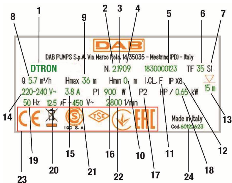
Fig.4 Data plate
