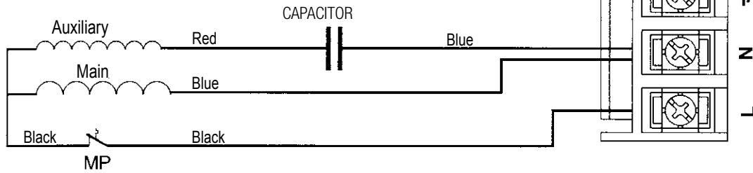
Overload protection inside the winding - MEC 63-71 M
