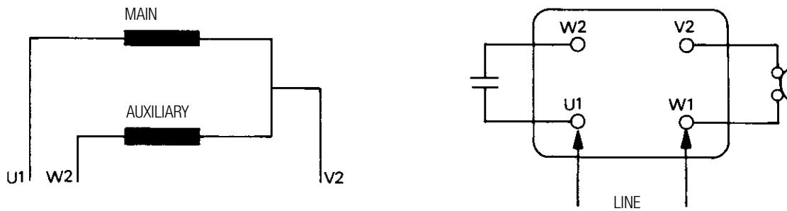
Overload protection inside the terminal board - MEC 80 M
